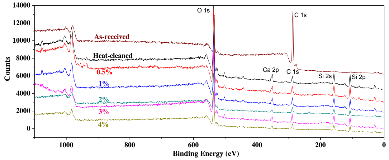
Figure 1 XPS spectra for differently treated glass fiber
